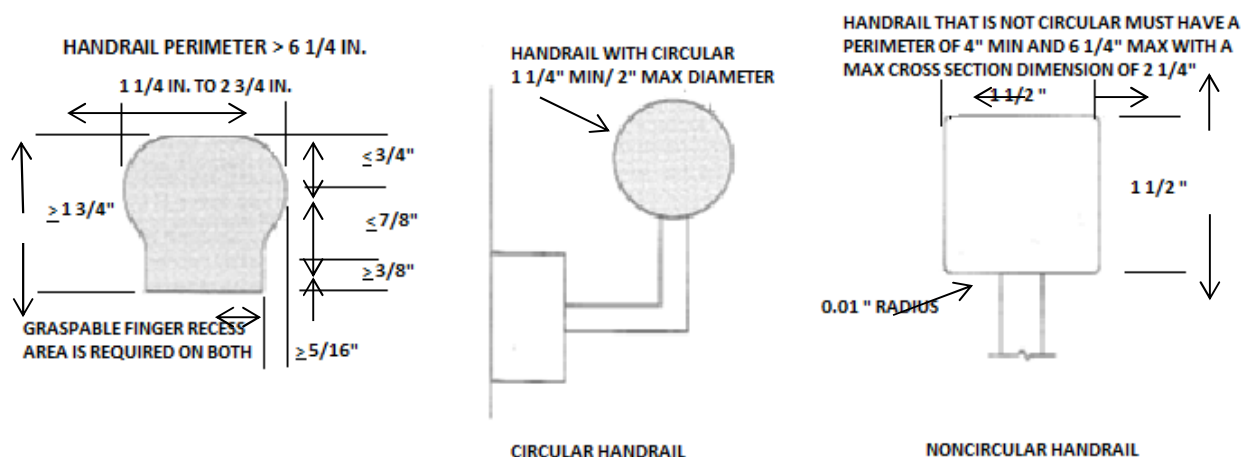
Figure 1: Acceptable handrail designs. Other shapes may be acceptable if they provide an equivalent gripping surface.
