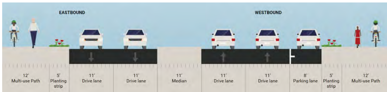
Plate 10 Option H – Class I Multi-Use Path
