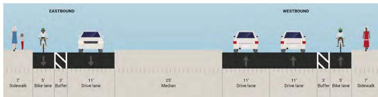
Plate 2 Option A – Widen Dublin Boulevard to the South
