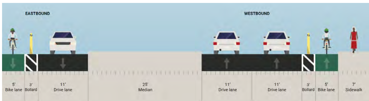
Plate 7 Option F – Class IV Separated Bikeway Option
