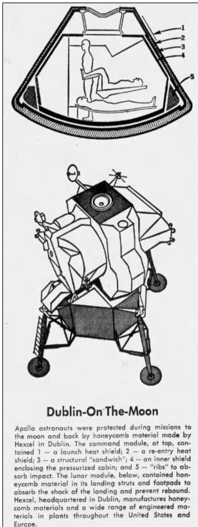
Plate 8: Diagrams showing where Hexcel honeycomb was utilized on the Apollo 11 lunar landing module (Source: Contra Costa Times 1967 March 26).
