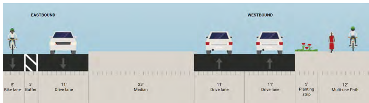
Plate 4 Option C – Westbound Only Class I Multi-Use Path
