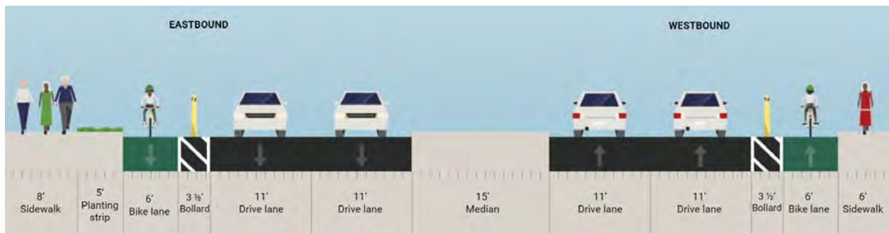
Plate 11 Option I – Class IV
