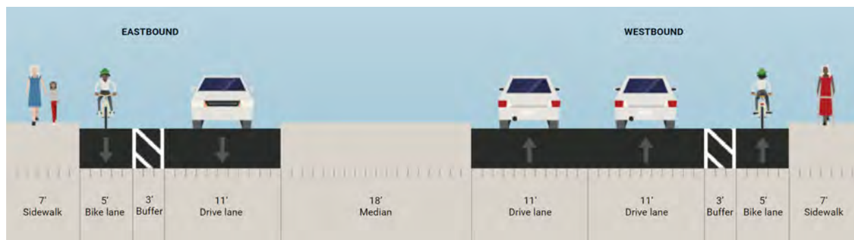
Plate 3 Option B – Narrow the Median
