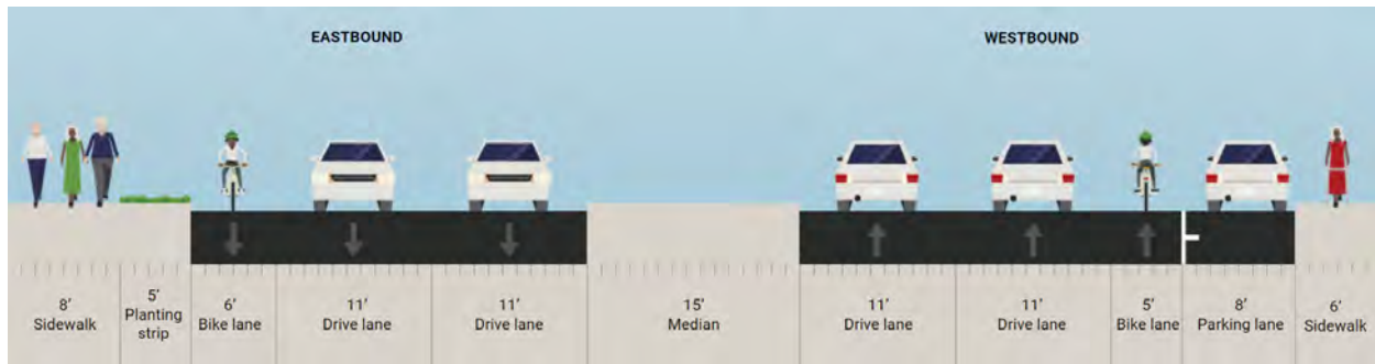
Plate 8 Existing Cross-Section of Dublin Boulevard between Donlon Way and Hansen Drive
