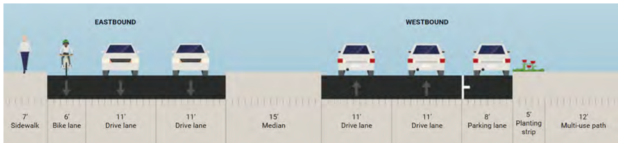
Plate 9 Option G – Westbound Only Class I Multi-Use Path
