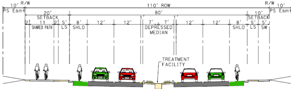
Figure 5. Typical Street Section with bioretention treatment in the median
